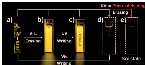
Figure 4. Reversible fluorescence image of the SS-TFMBE/TFM-BTE organogel system in a quartz cell ( \lambda_{\text{ex}} = 365 nm). a) Writing, b) erasing, c) rewriting, d) re-erasing, and e) erasing by heat-sol state. The dark region represents the irradiated area (with 300 nm UV light). White dashed lines are shown around d) and e) for clarity.
